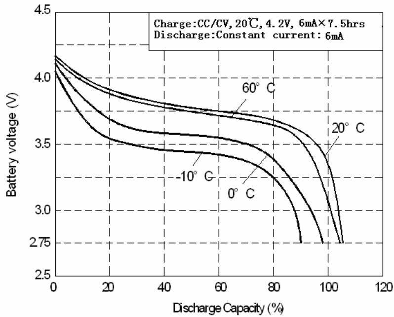
Discharging Characteristics at Various Temp.
